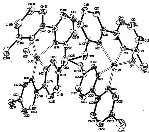
Fig. 2 The structure of the cation [\text{Cu}^{\text{II}}\text{L}^{56}(\text{OH})(\text{H}_2\text{O})]^{3+} with the atom numbering scheme. Thermal ellipsoids are drawn at 50% probability.
